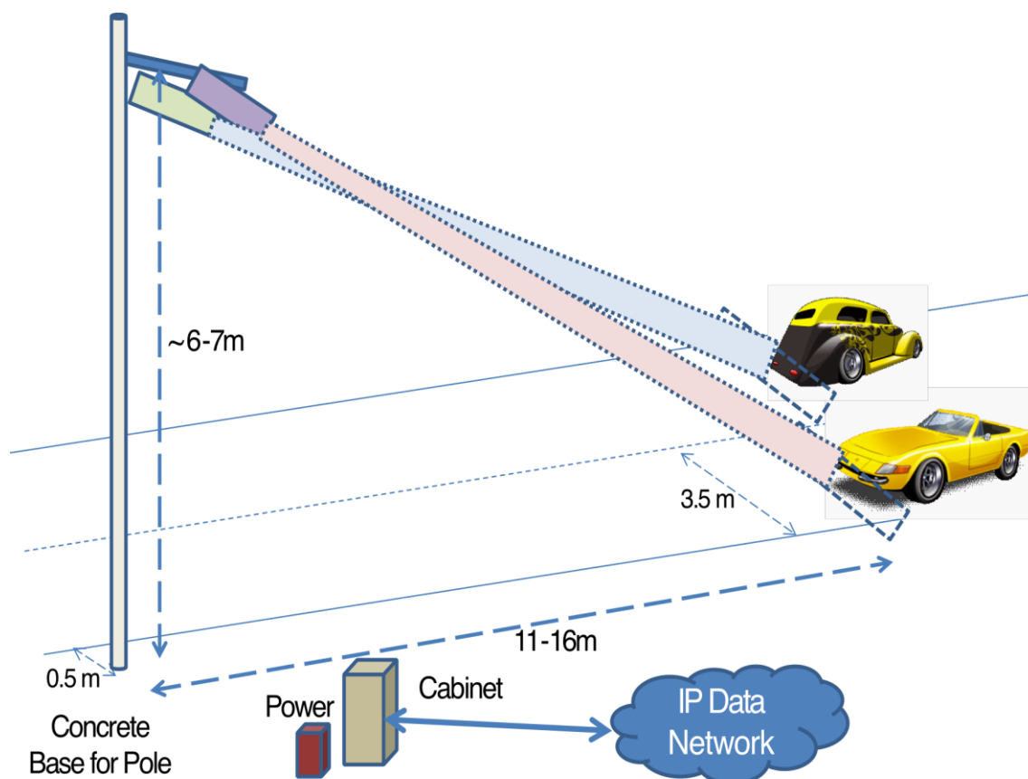
Figure 10.5: Typical layout of number plate reader and enforcement cameras in London (above) and example of implementation (below)
